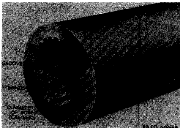
Fig 1 Rifling Details
